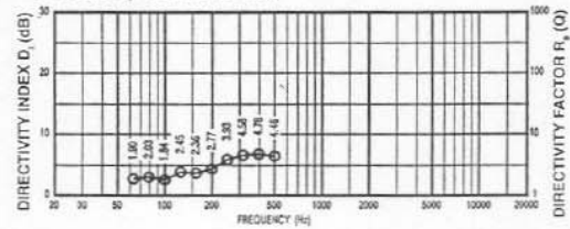
FIGURE 6 — Directivity vs. Frequency
